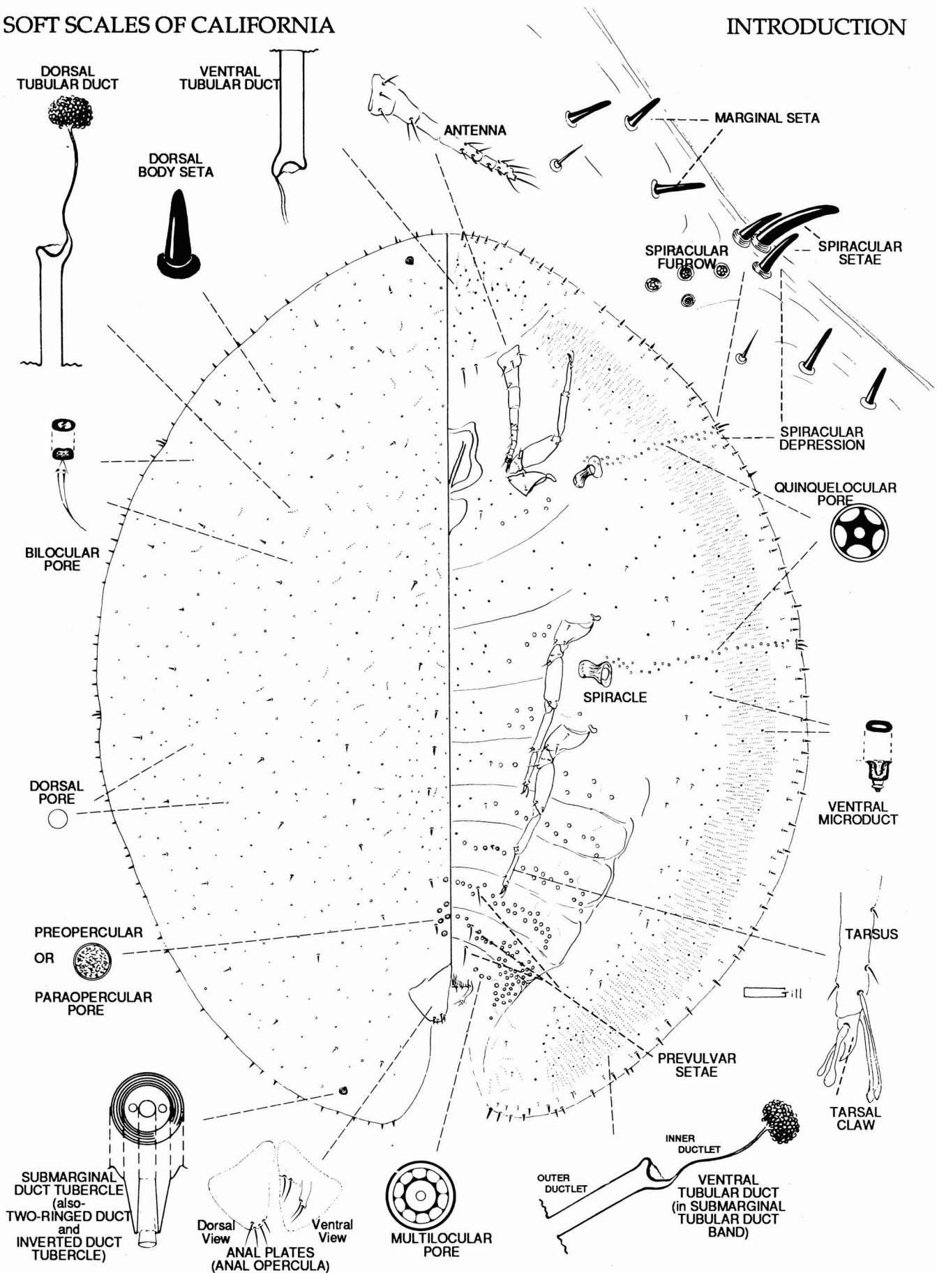
Fig. 2: Morphological structures of the Coccidae
